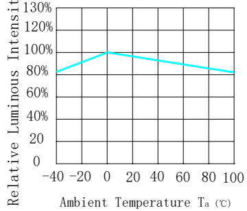
Fig.4 Relative Intensity Vs Ambient Temperature
